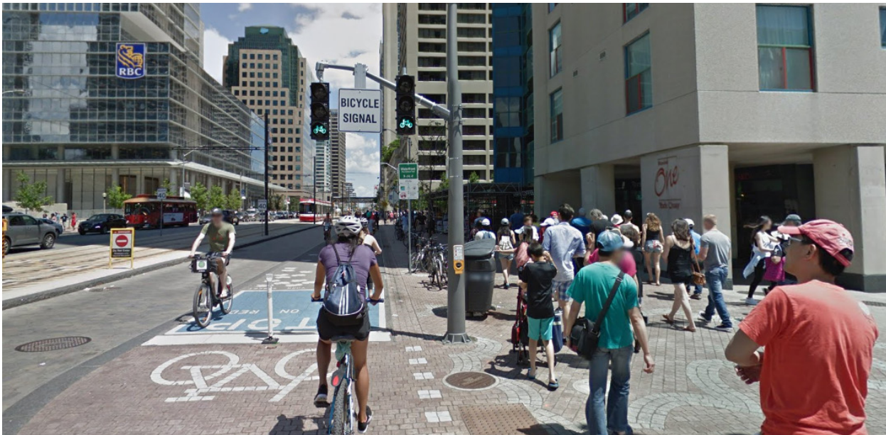
Bicycle-specific signals, seen here in Toronto, are easier for cyclists to see when installed at the same height as pedestrian signals. Source: Google Maps
