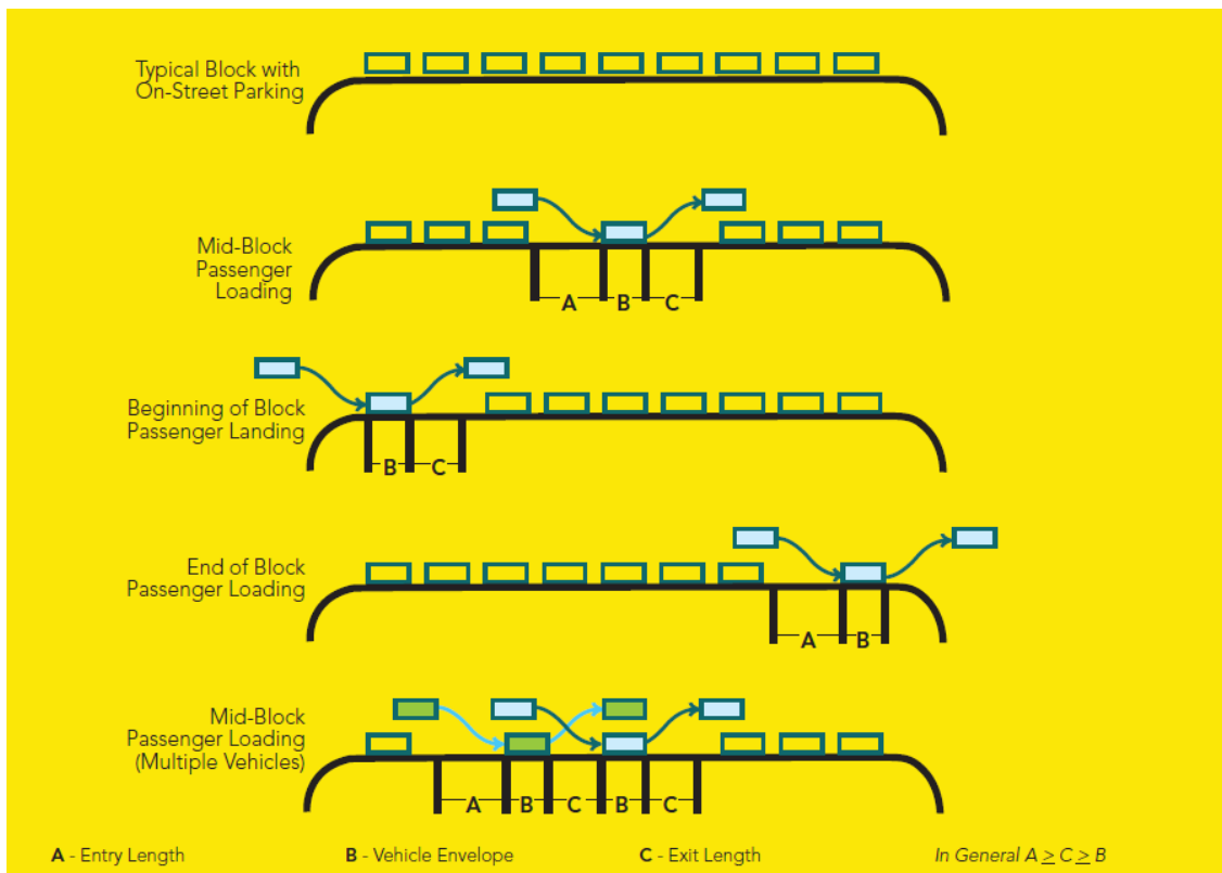
This diagram demonstrates the curb space required for passenger loading in different configurations. Source: ITE
