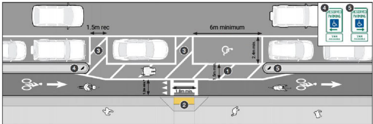
Accessible On-Street Motor Vehicle Parking Example. Source: MassDOT
