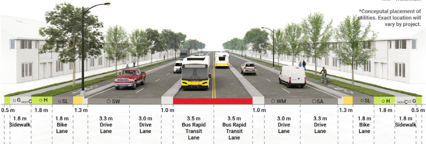
Typical Transitioning Avenue Cross Section with centre-running BRT at mid-block (36m ROW).
