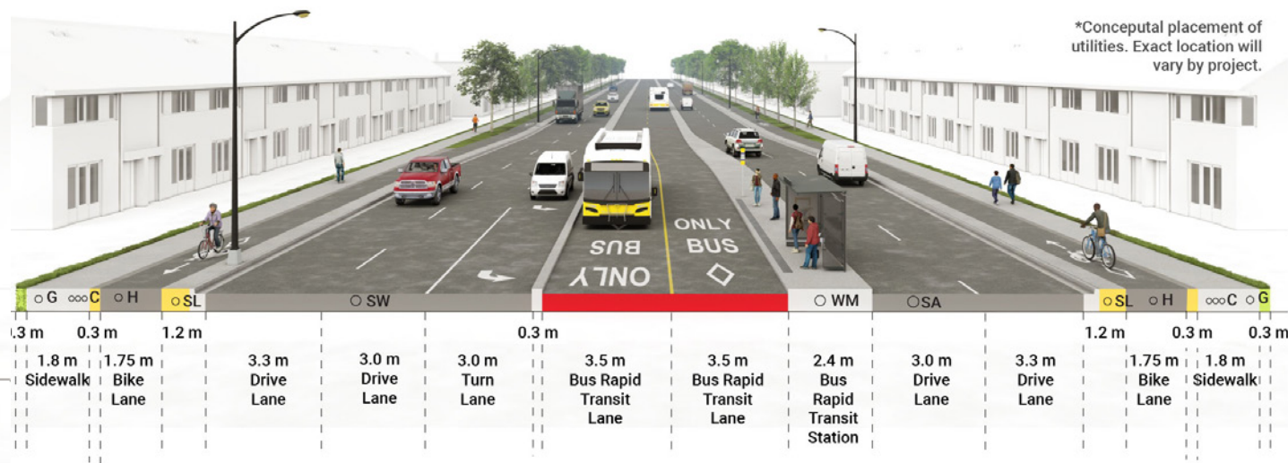
Typical Transitioning Avenue Cross Section with centre-running BRT approaching intersection and transit stop (36m ROW).
