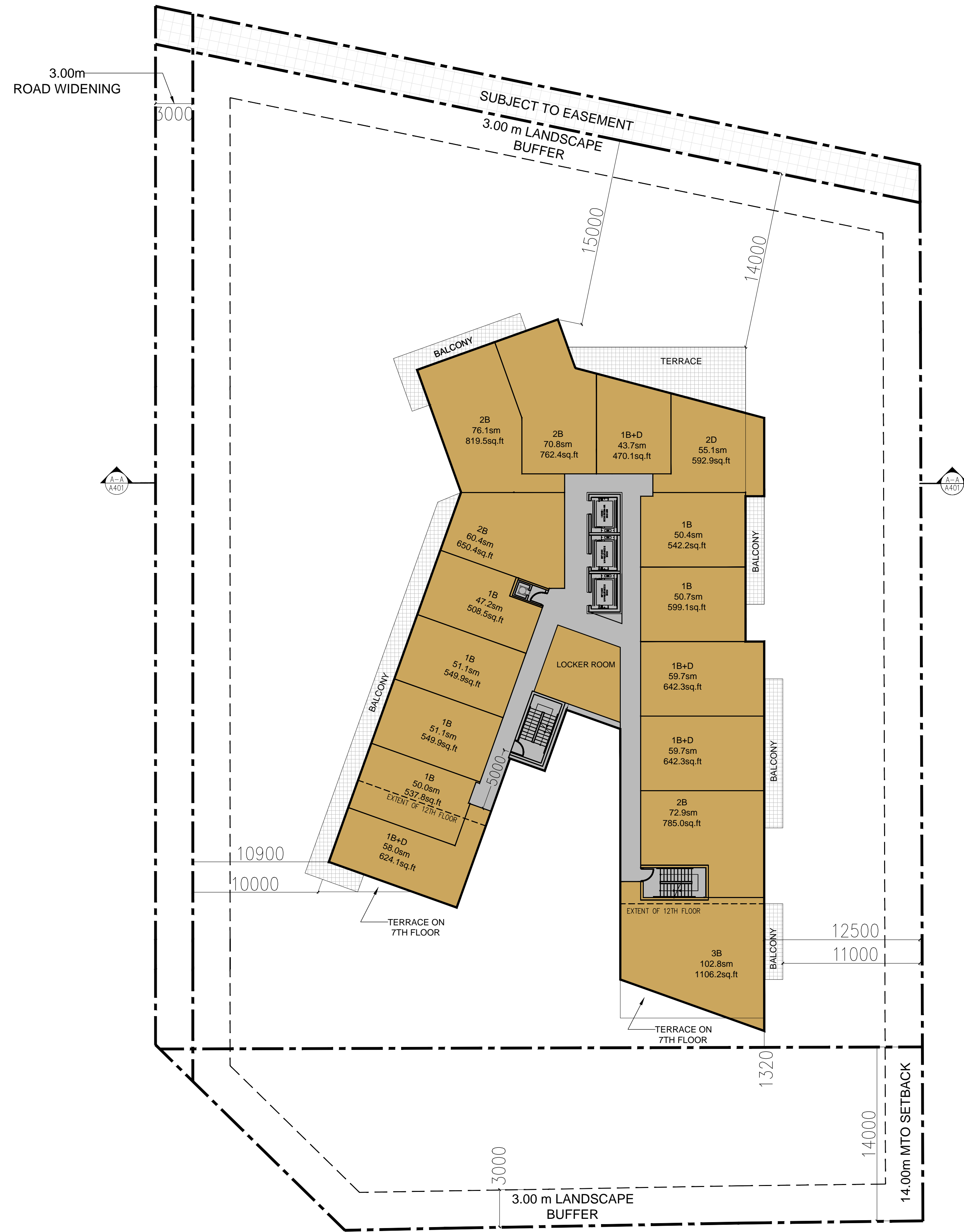
11TH FLOOR PLAN
