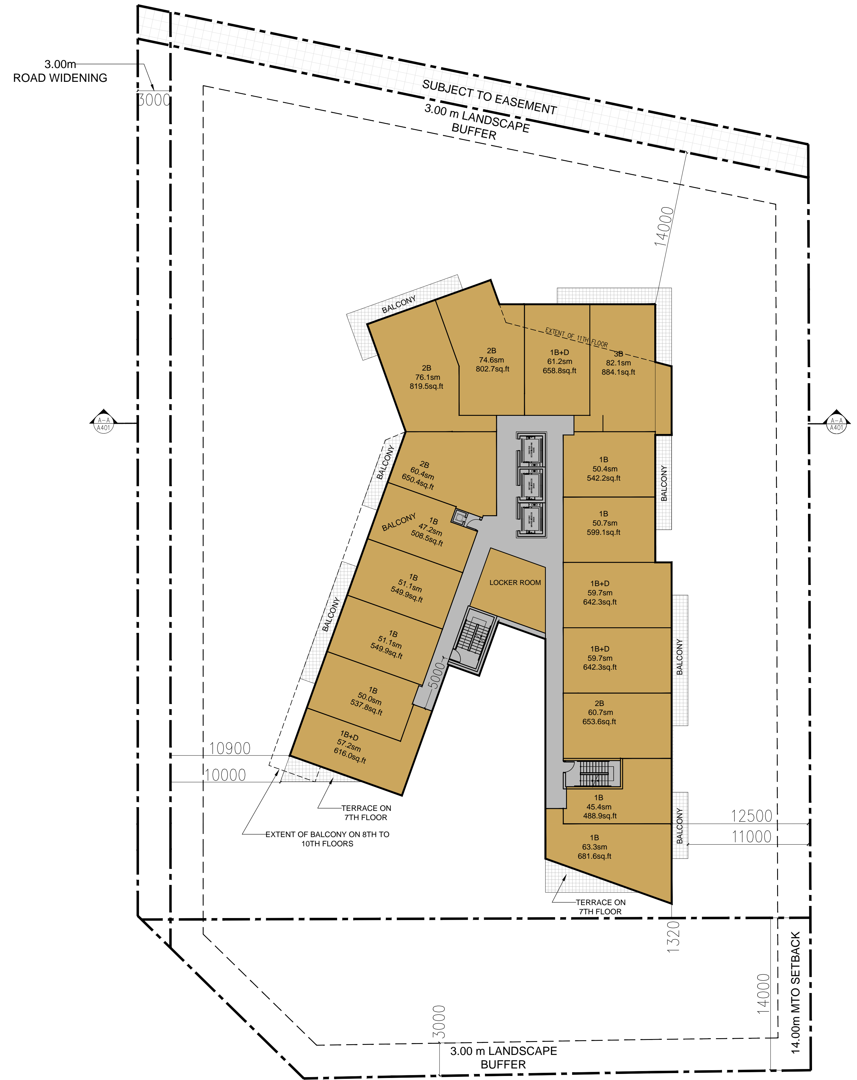
7TH TO 10TH FLOOR PLANS
