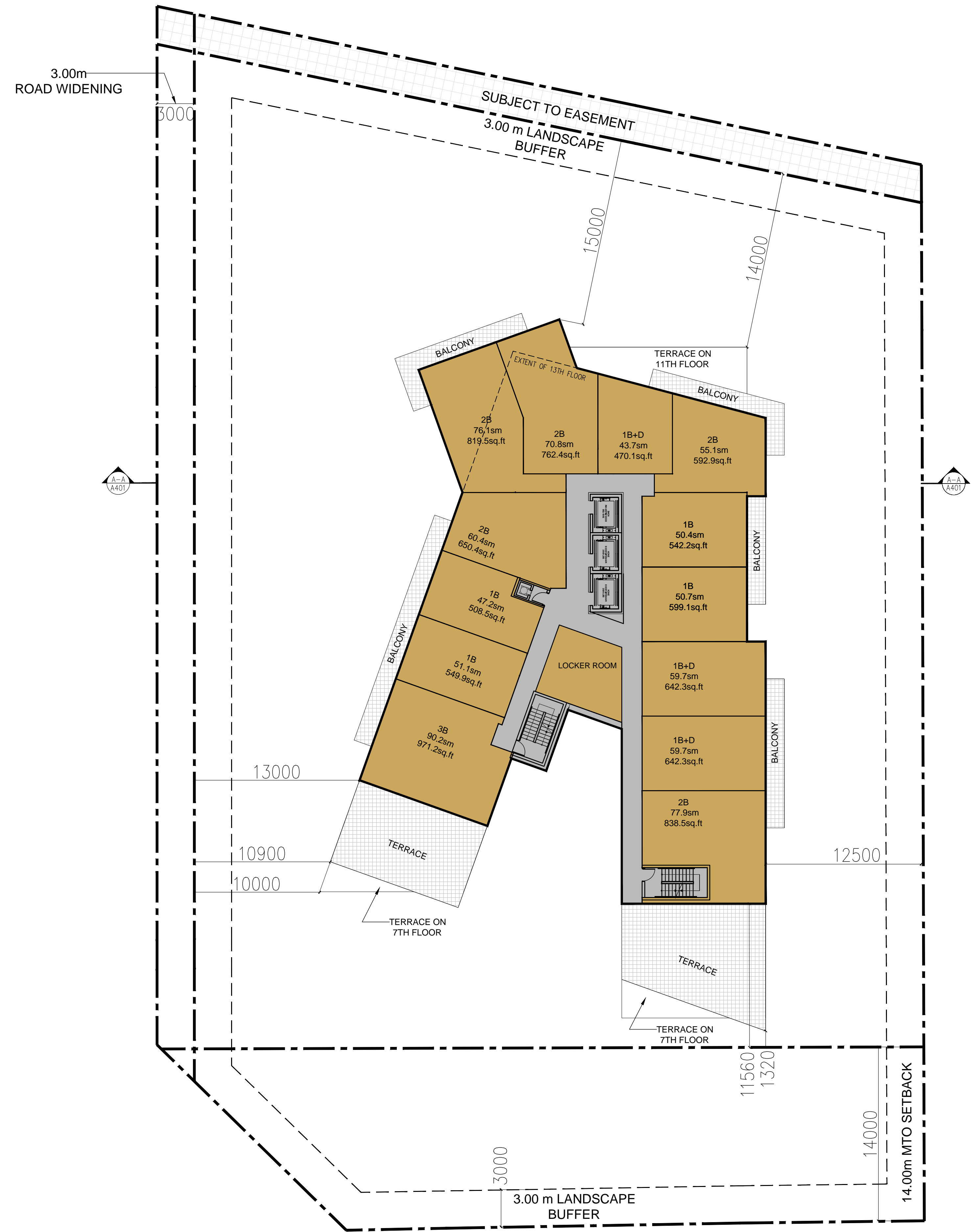
12TH FLOOR PLAN
