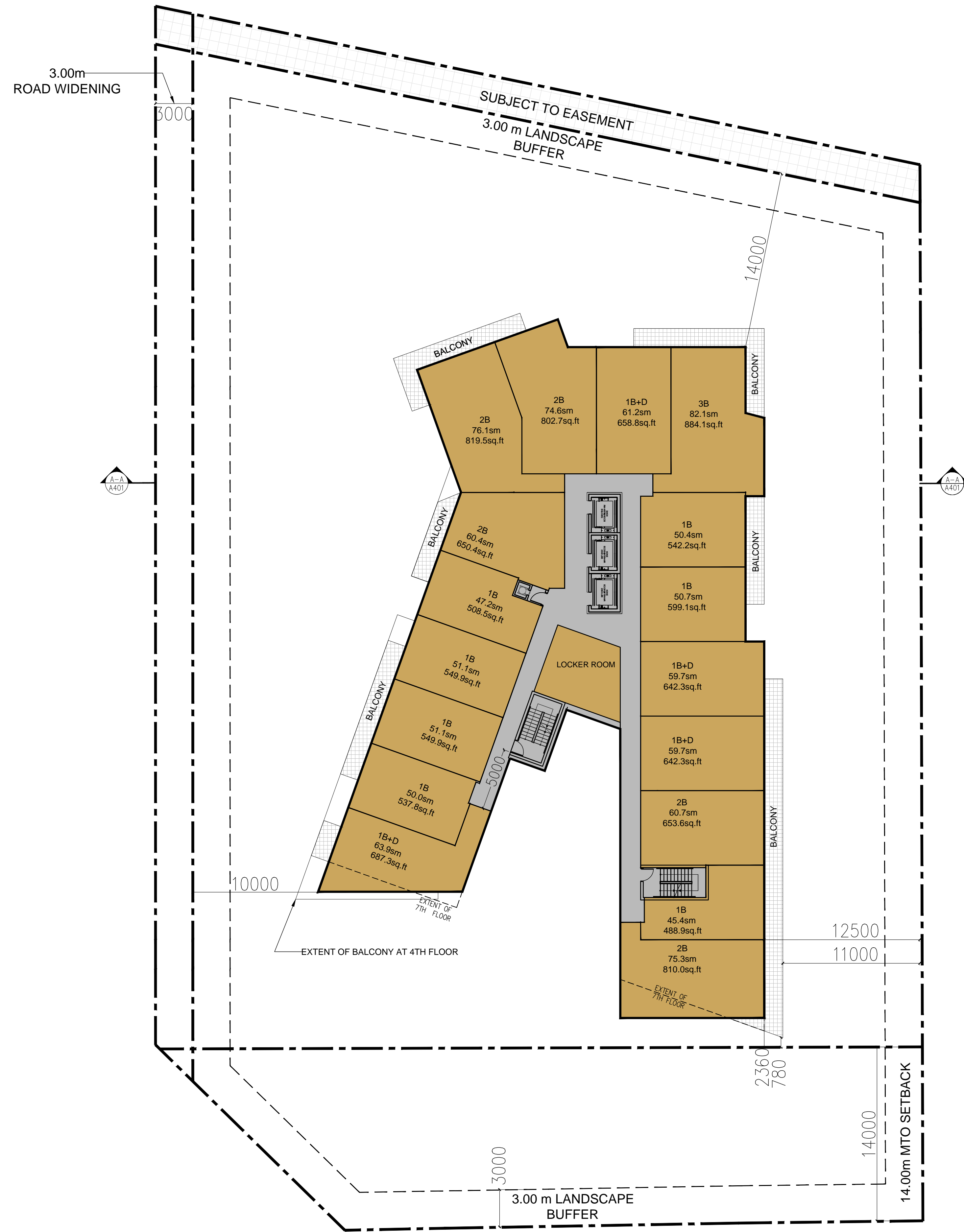
5TH AND 6TH FLOOR PLANS
