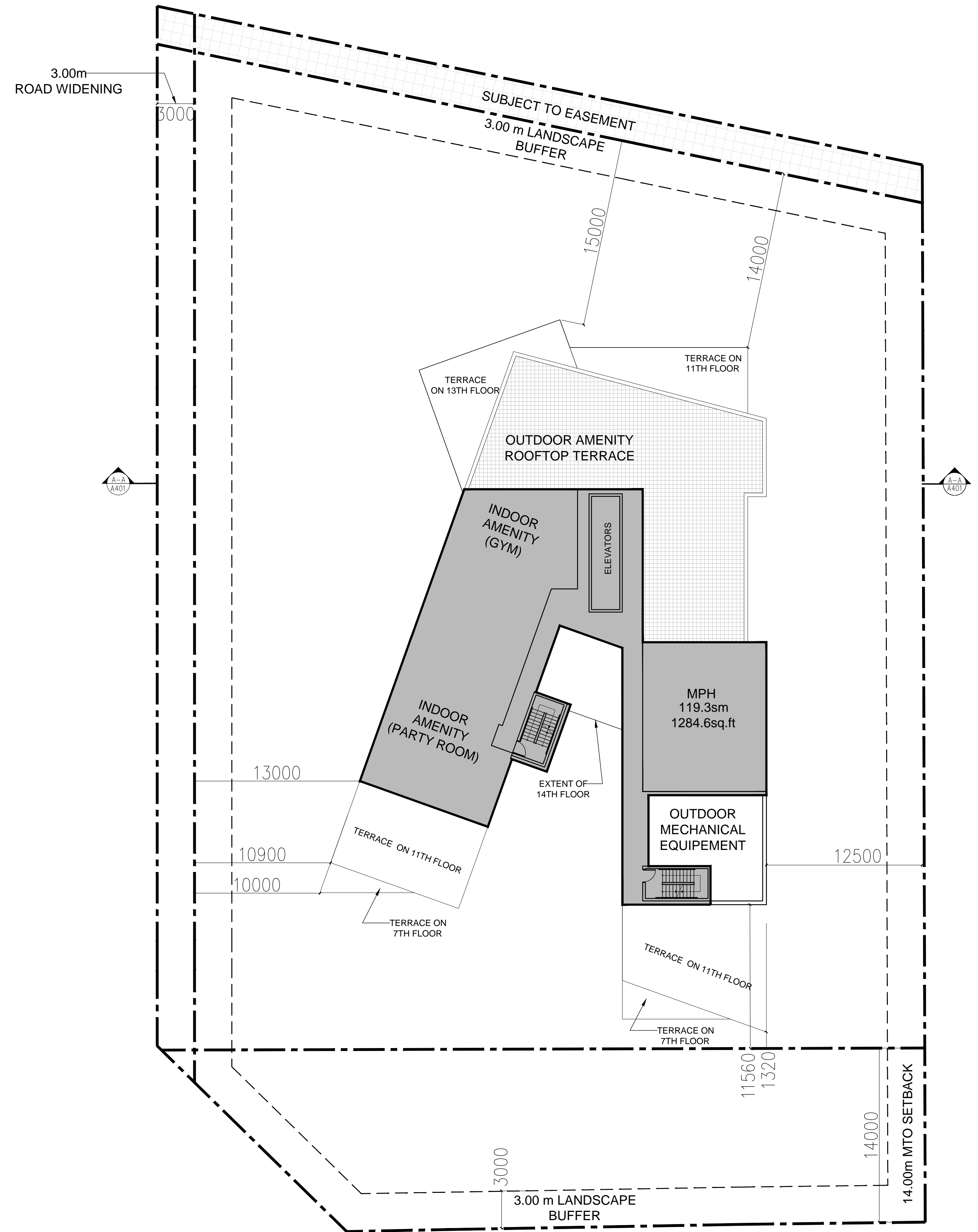
AMENITY AND MPH FLOOR PLAN
