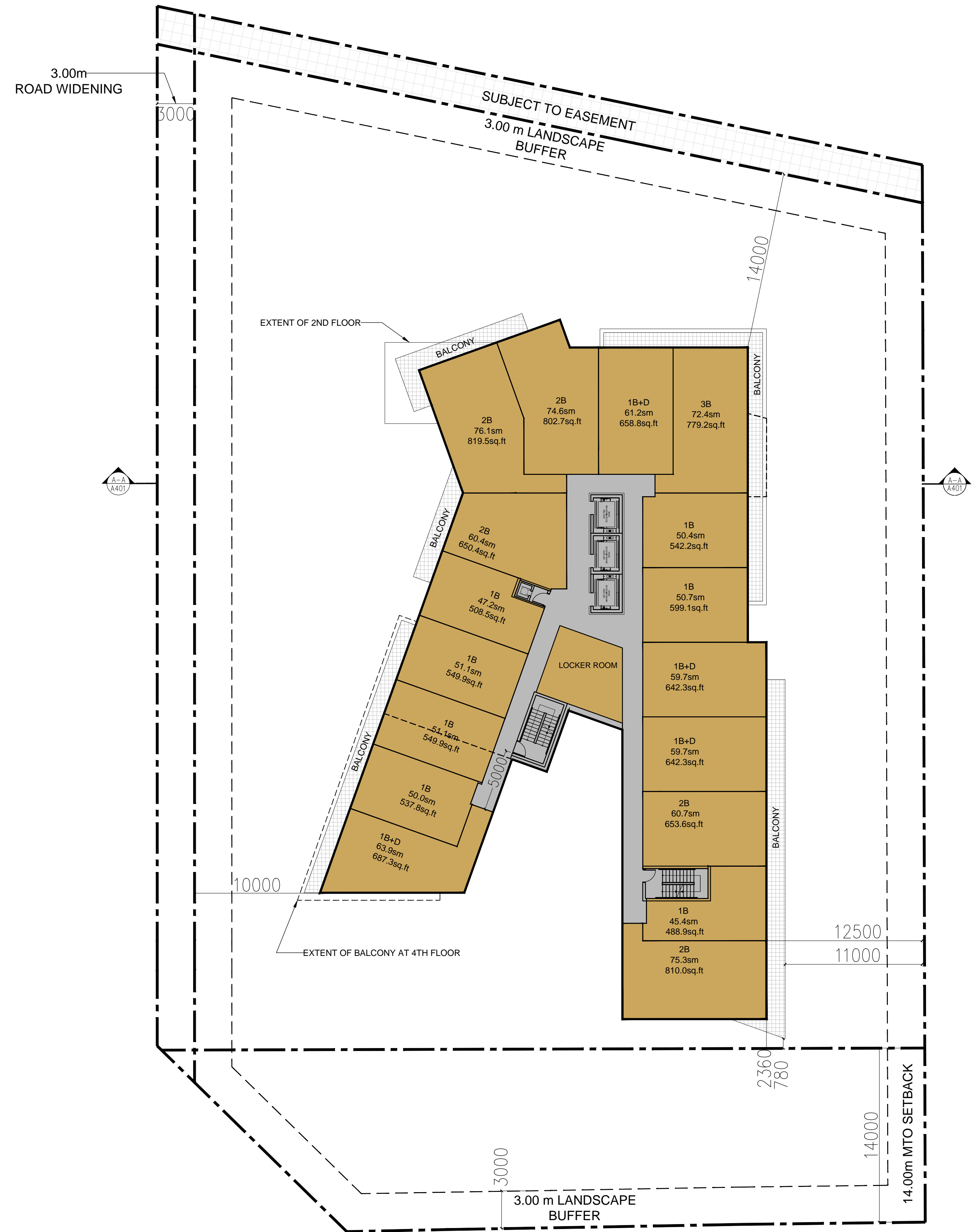
3RD & 4TH FLOOR PLANS
