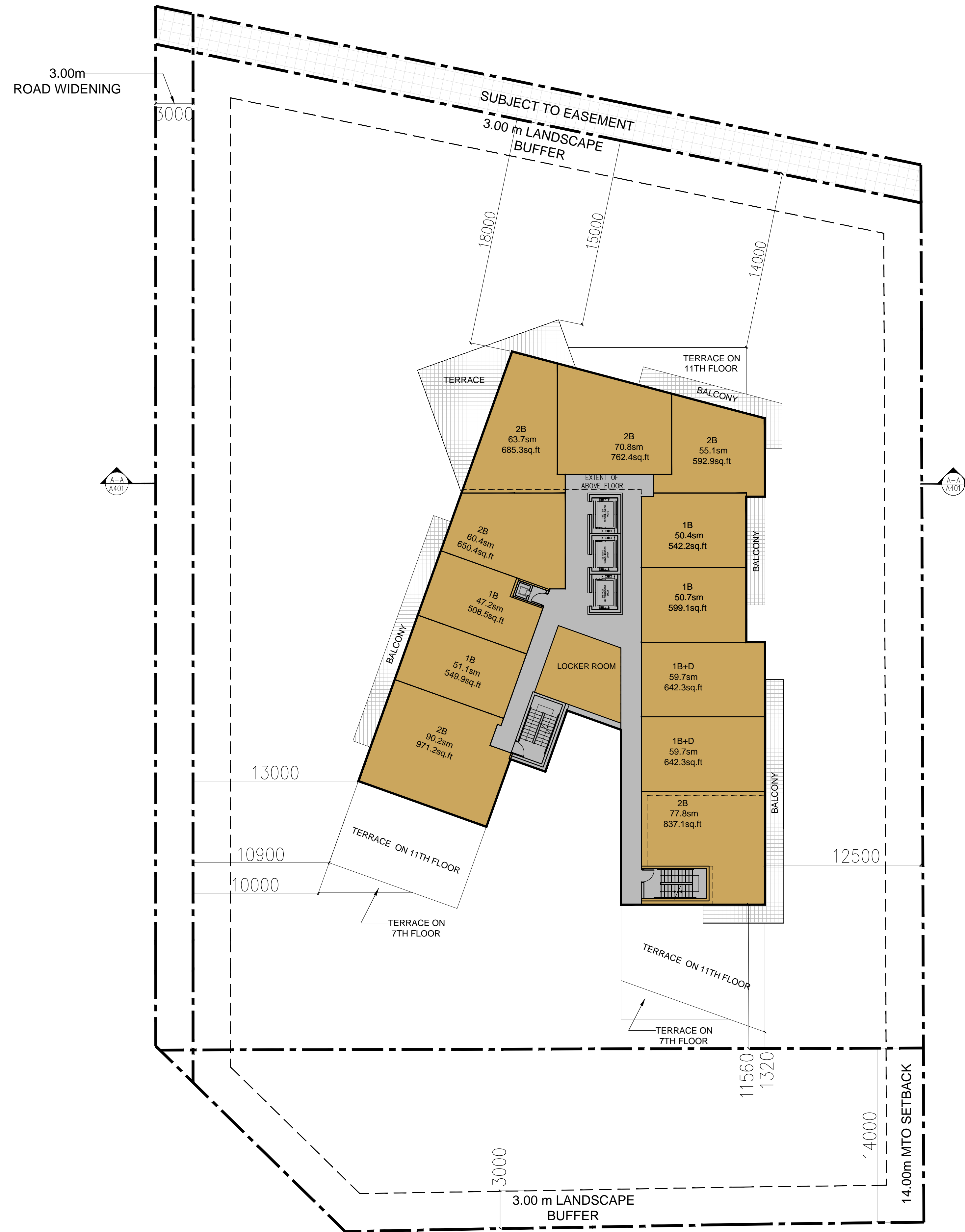
13TH & 14TH FLOOR PLANS
